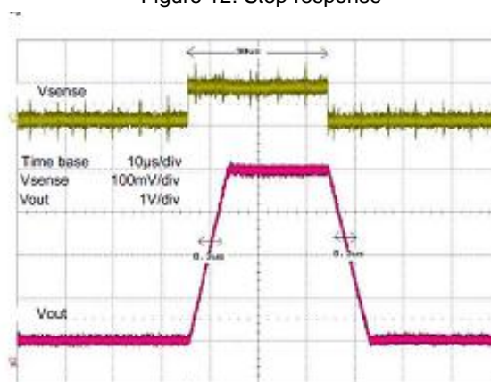
Figure 12: Step response
