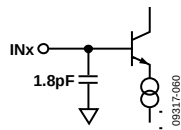
Figure 58. Analog Input
