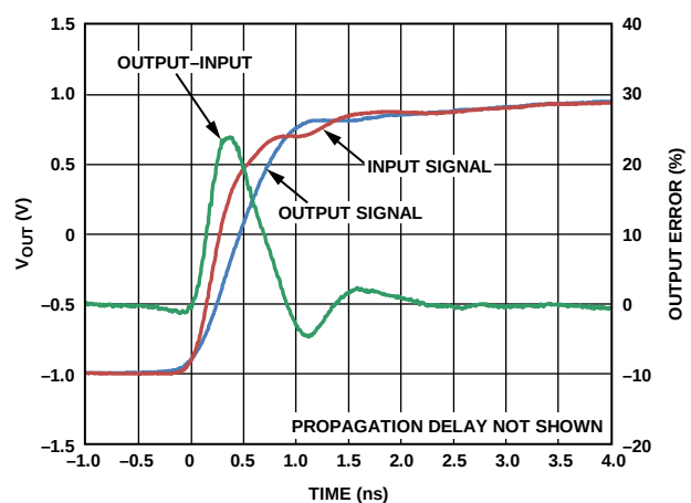
Figure 24. ADV3225 Settling Time
