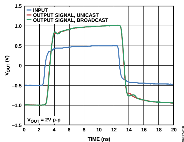
Figure 18. ADV3225 Large Signal Pulse Response
