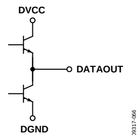
Figure 64. Logic Output
