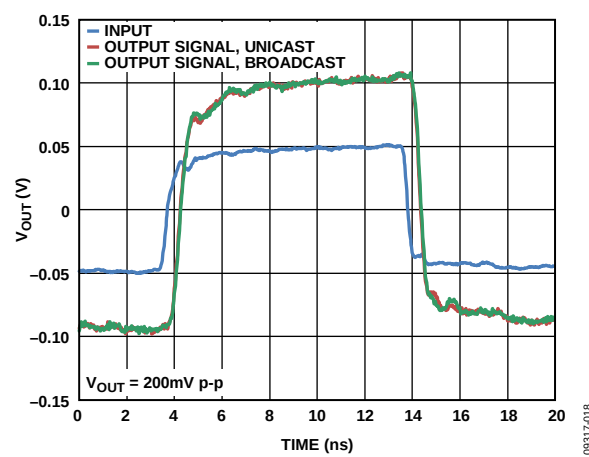
Figure 17. ADV3225 Small Signal Pulse Response
