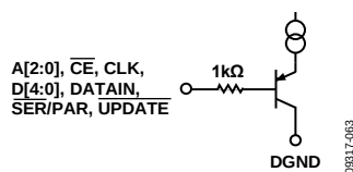
Figure 61. Logic Input
