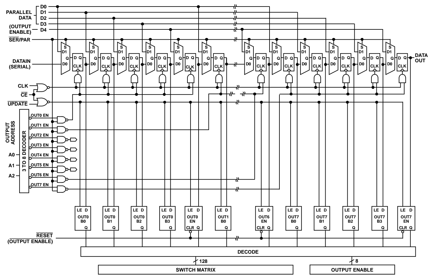
Figure 6. Logic Diagram
