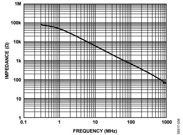
Figure 40. ADV3225 Output Impedance, Disabled
