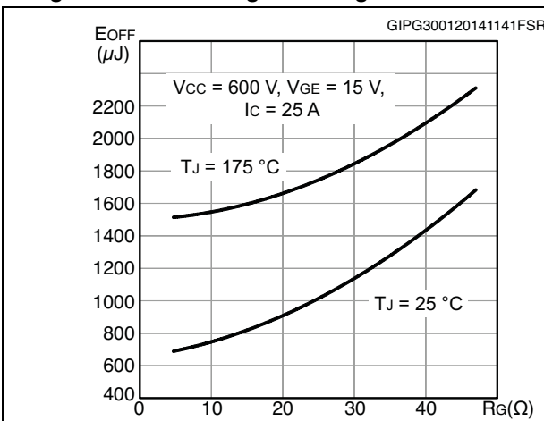
Figure 16. Switching loss vs gate resistance
