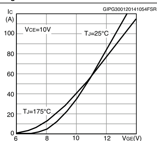
Figure 9. Transfer characteristics
