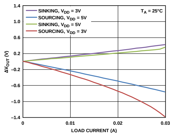
Figure 29. Headroom/Footroom vs. Load Current
