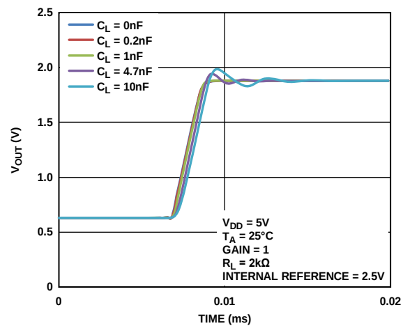
Figure 31. Settling Time vs. Capacitive Load, Gain = 1
