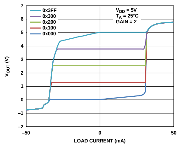
Figure 30. Source and Sink Capability, Gain = 2
