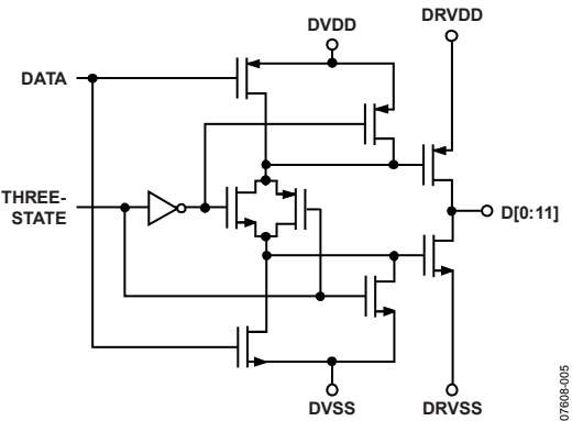
Figure 10. Data Outputs
