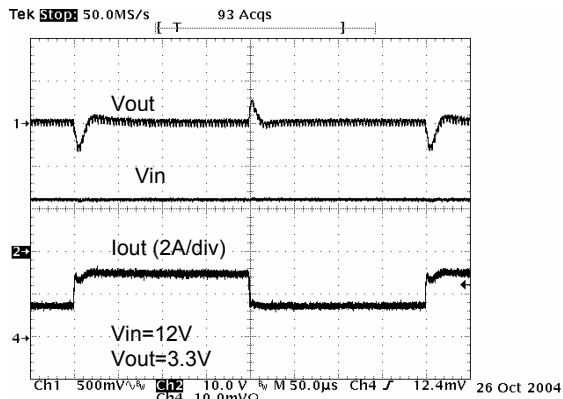
Figure 3. Load Step Response: 1.5->3A
