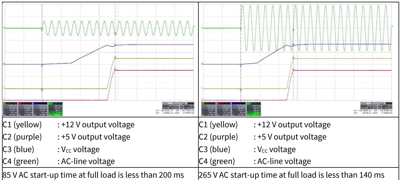
Figure 21 Start-up
