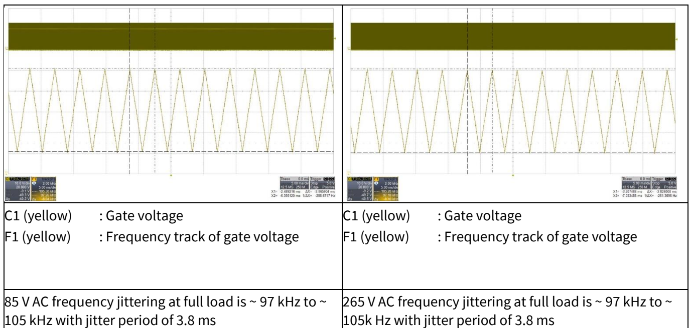
Figure 24 Frequency jittering
