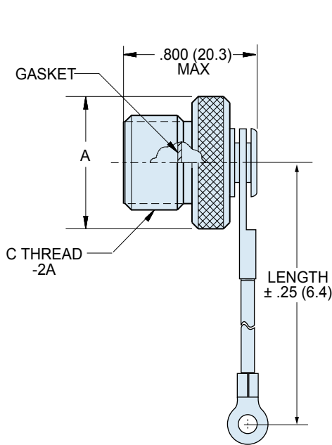
667-217 Plug Cover
