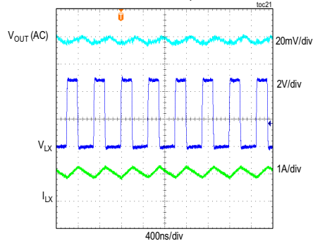
LV BUCK STEADY-STATE SWITCHING WAVEFORMS ( V_{IN} = 5V , V_{OUT} = 1.8V , MODE = PWM LOAD = 1A)
