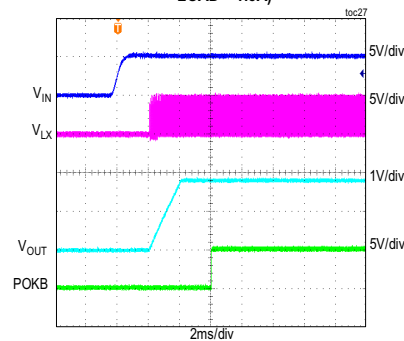
LV BUCK STARTUP FROM INPUT ( V_{IN} = 5V , V_{OUT} = 1.8V , MODE = PWM LOAD = 1.5A)
