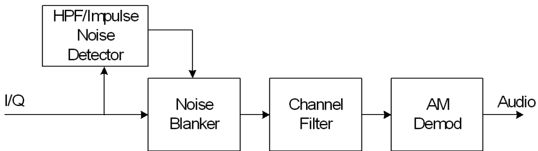
Figure 20. Illustration of Noise Blanker in AM Signal Path.
