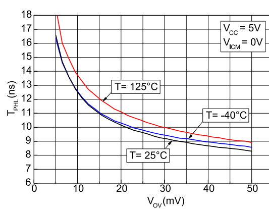
Figure 16: Propagation delay vs. overdrive with negative transition, V_{CC} = 5\text{V}
