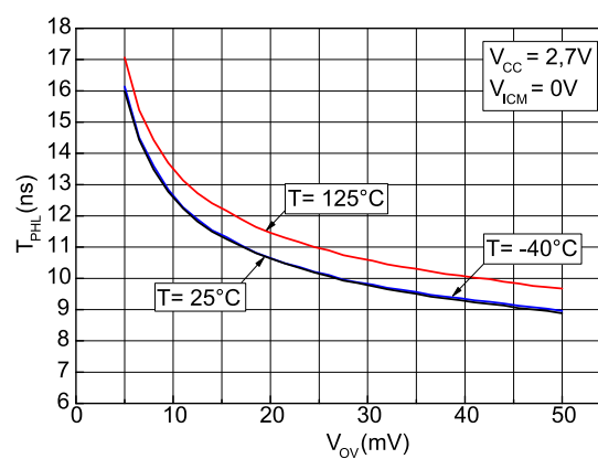
Figure 14: Propagation delay vs. overdrive with negative transition, V_{CC} = 2.7\text{V}
