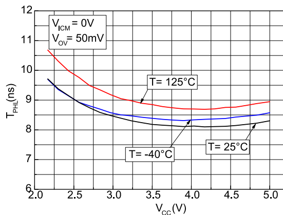
Figure 12: Propagation delay vs. power supply voltage with negative transition
