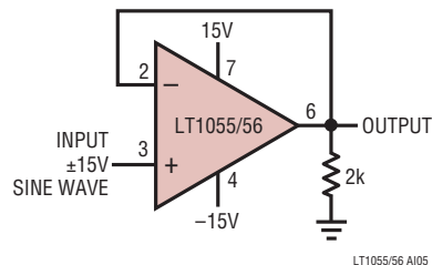
Voltage Follower with Input Exceeding the Negative Common Mode Range
