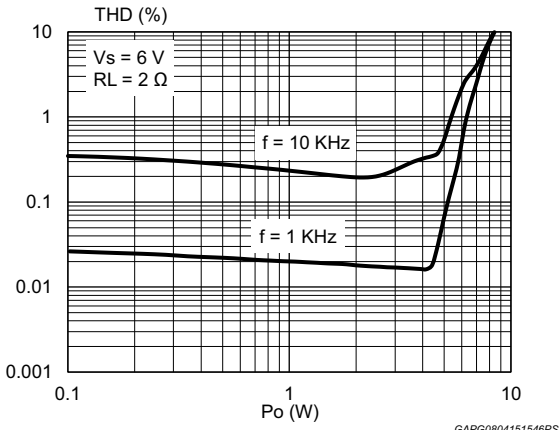
Figure 13. Distortion vs. output power (2 \Omega , V_s = 6 V)
