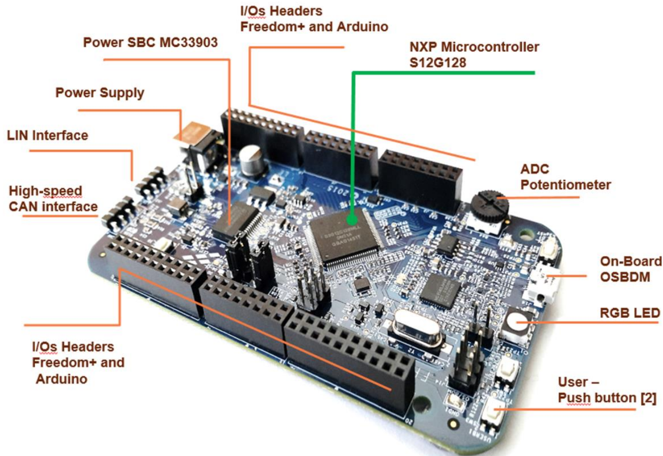
DEVKIT-S12G128 Features
