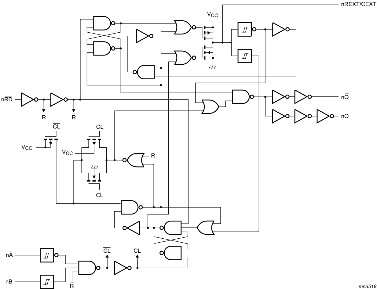
Fig 4. Logic diagram
