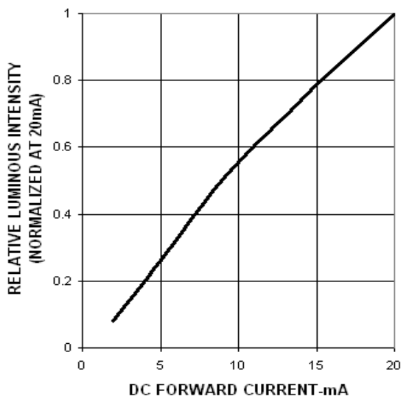
Figure 2: Relative Luminous Intensity vs. Forward Current.
