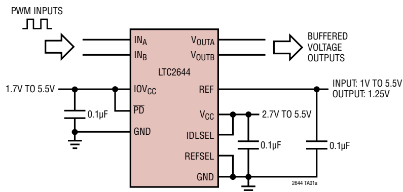
2-Channel PWM to Voltage Output DAC
