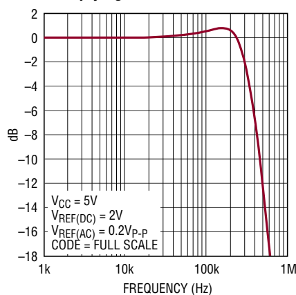
Multiplying Bandwidth
