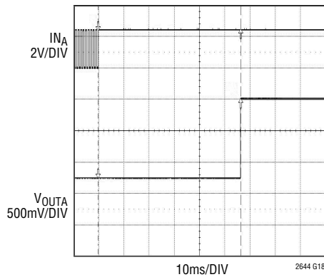
Entering Idle Mode Full-Scale from Mid-Scale ( IDLSEL = \text{GND} )
