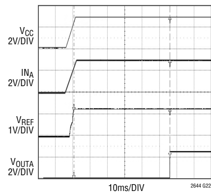
Power-On-Reset to Idle Mode Full-Scale ( IDLSEL = \text{GND} )
