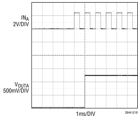
Exiting Idle Mode Zero-Scale to Mid-Scale ( IDLSEL = \text{GND} )
