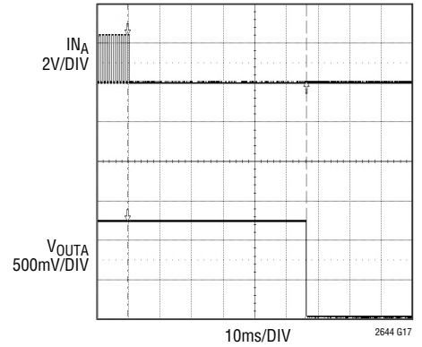
Entering Idle Mode Zero-Scale from Mid-Scale ( IDLSEL = \text{GND} )
