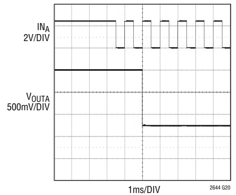
Exiting Idle Mode Full-Scale to Mid-Scale ( IDLSEL = \text{GND} )
