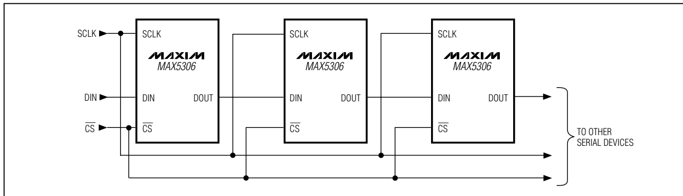
Figure 5. Daisy-Chaining MAX5306s
