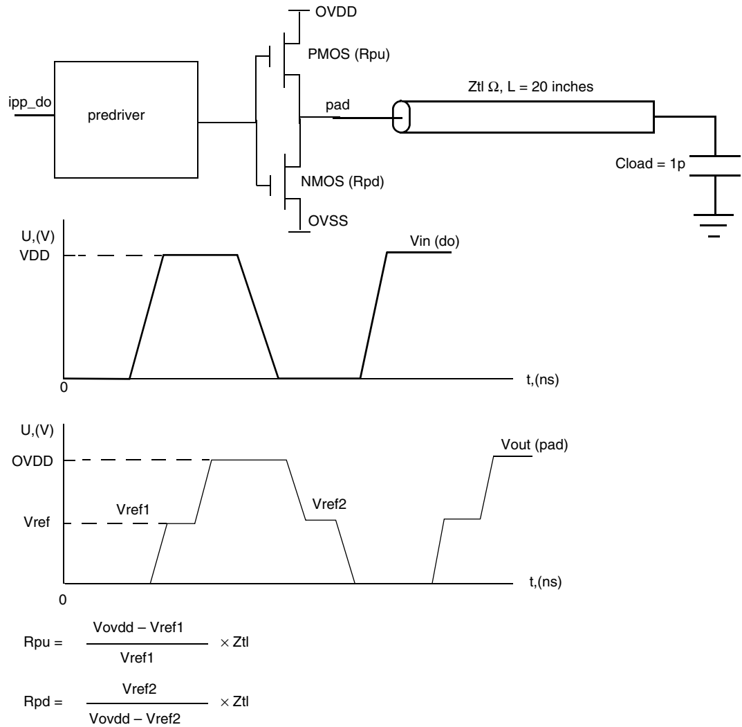
Figure 7. Impedance Matching Load for Measurement
