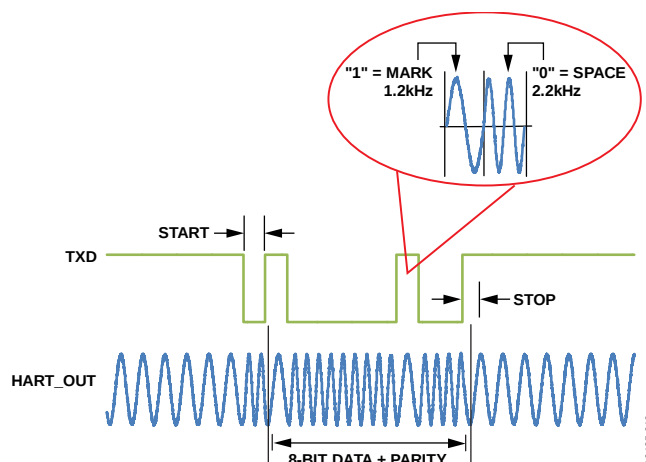
Figure 19. AD5700/AD5700-1 Modulator Waveform
