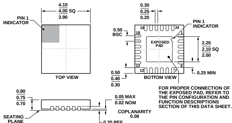
Figure 33. 24-Lead Lead Frame Chip Scale Package [LFCSP_WQ] 4 mm × 4 mm Body, Very Thin Quad (CP-24-10) Dimensions shown in millimeters
