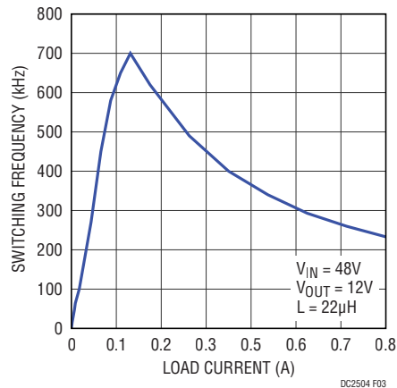
Figure 3. Switching Frequency vs Load Current
