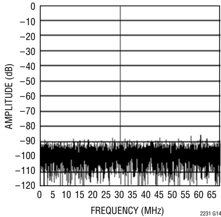
LTC2231: 8192 Point FFT, f_{IN} = 30\text{MHz} , -1dB, 2V Range
