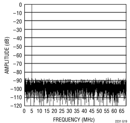
LTC2231: 8192 Point FFT, f_{IN} = 140\text{MHz} , -1dB, 1V Range
