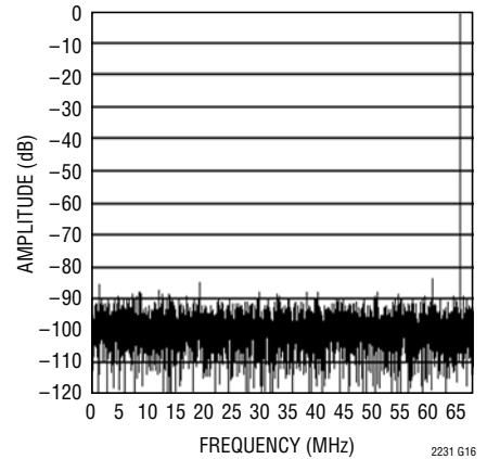
LTC2231: 8192 Point FFT, f_{IN} = 70\text{MHz} , -1dB, 2V Range
