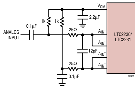
Figure 5. Single-Ended Drive
