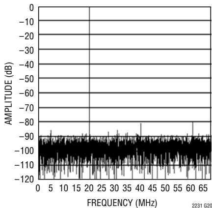
LTC2231: 8192 Point FFT, f_{IN} = 250\text{MHz} , -1dB, 2V Range
