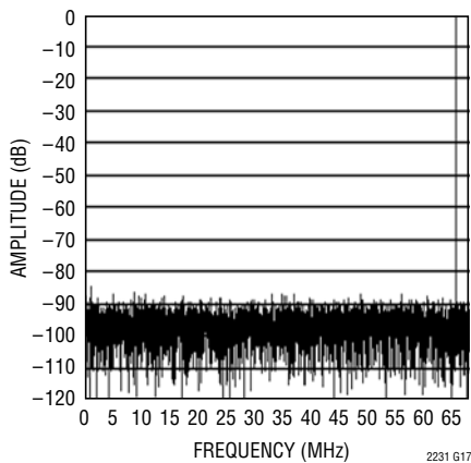
LTC2231: 8192 Point FFT, f_{IN} = 70\text{MHz} , -1dB, 1V Range
