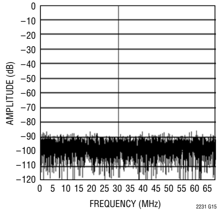
LTC2231: 8192 Point FFT, f_{IN} = 30\text{MHz} , -1dB, 1V Range
