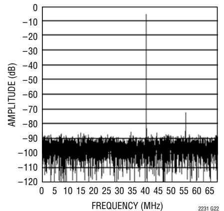
LTC2231: 8192 Point FFT, f_{IN} = 500\text{MHz} , -6dB, 1V Range
