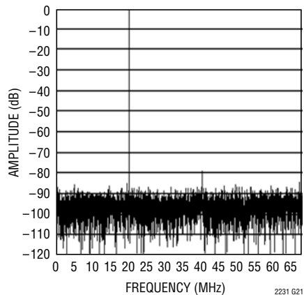
LTC2231: 8192 Point FFT, f_{IN} = 250\text{MHz} , -1dB, 1V Range
