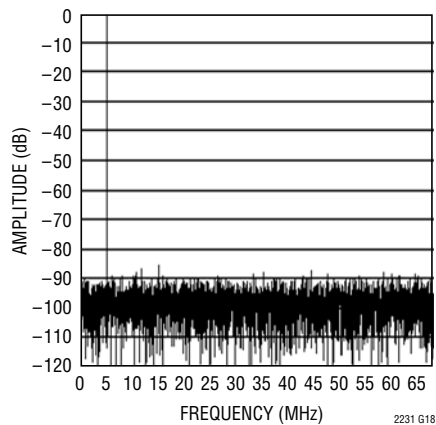
LTC2231: 8192 Point FFT, f_{IN} = 140\text{MHz} , -1\text{dB} , 2\text{V} Range
