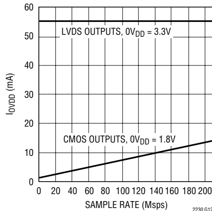
LTC2230: I_{OVD} vs Sample Rate, 5MHz Sine Wave Input, -1dB
