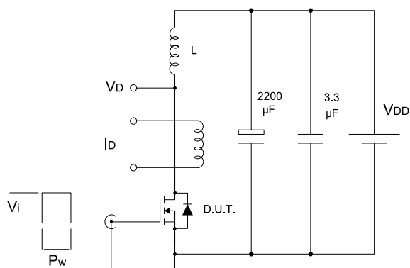
Figure 16: Unclamped inductive load test circuit
