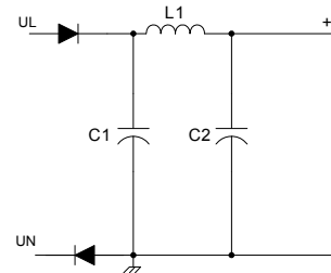
Figure 10: Half-Wave Rectifier
