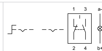
Wiring diagram 23
