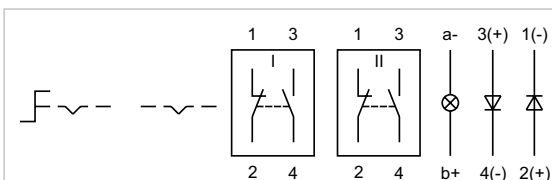
Wiring diagram 25
