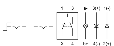
Wiring diagram 21
