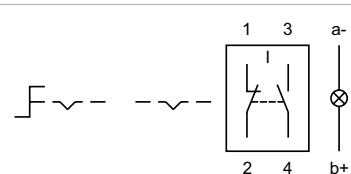
Wiring diagram 23
