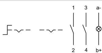
Wiring diagram 19
