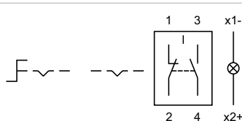
Wiring diagram 22
