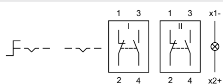
Wiring diagram 26
