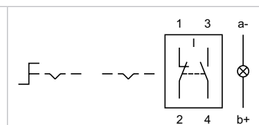
Wiring diagram 23
