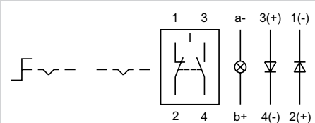
Wiring diagram 21
