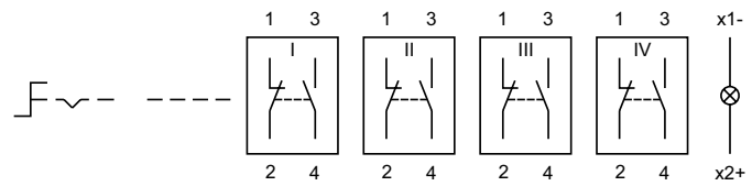
Wiring diagram 14
