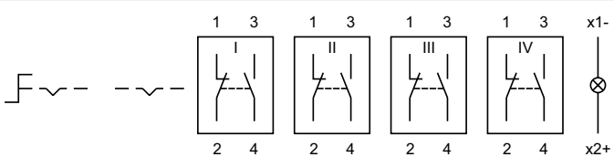
Wiring diagram 28
