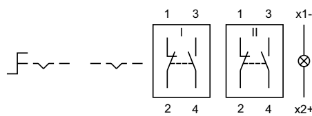
Wiring diagram 26
