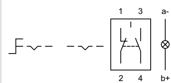
Wiring diagram 23
