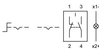
Wiring diagram 22
