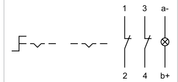
Wiring diagram 18
