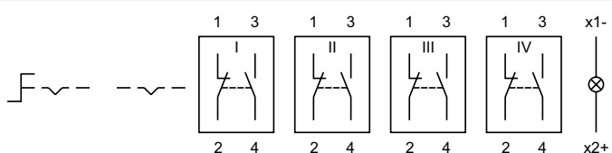
Wiring diagram 28
