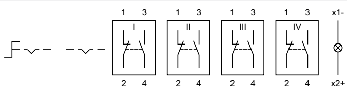
Wiring diagram 28
