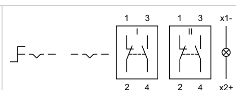
Wiring diagram 26
