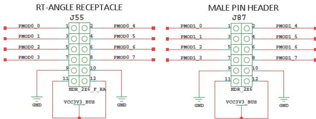
Figure 3-29: PMOD Connectors
