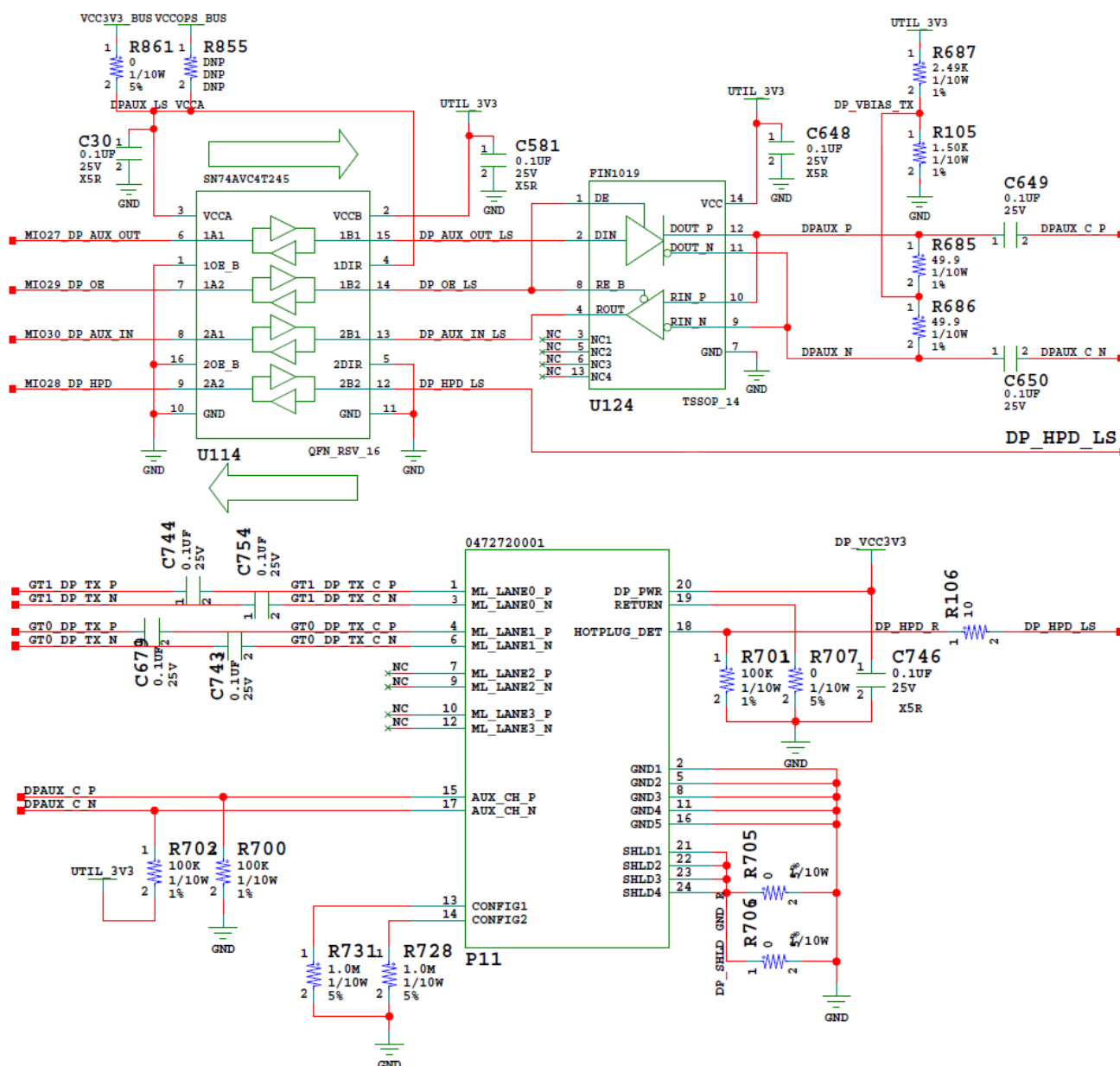
Figure 3-22: DisplayPort Circuit
