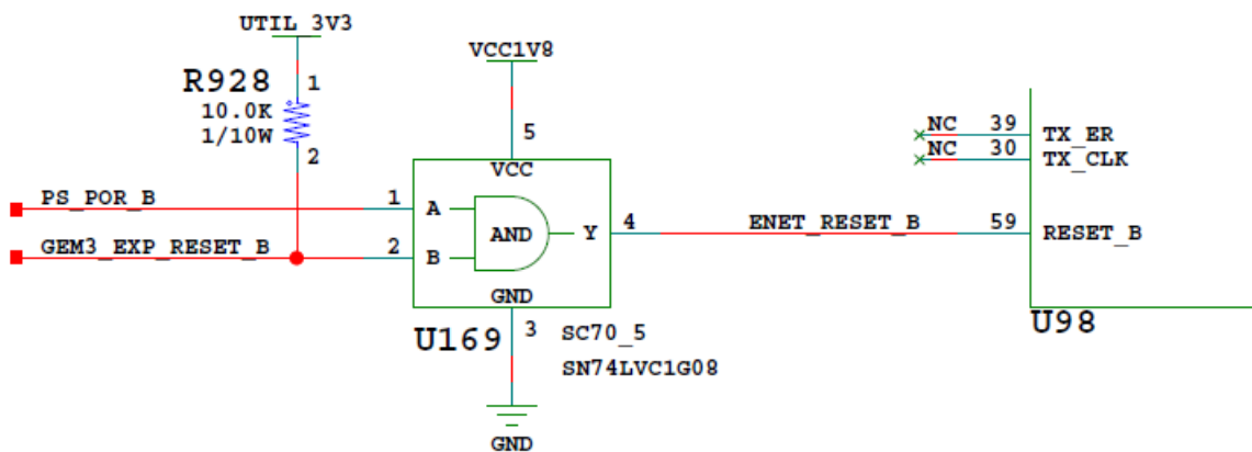
Figure 3-10: Ethernet PHY Reset Circuit
