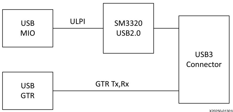
Figure 3-3: USB Interface
