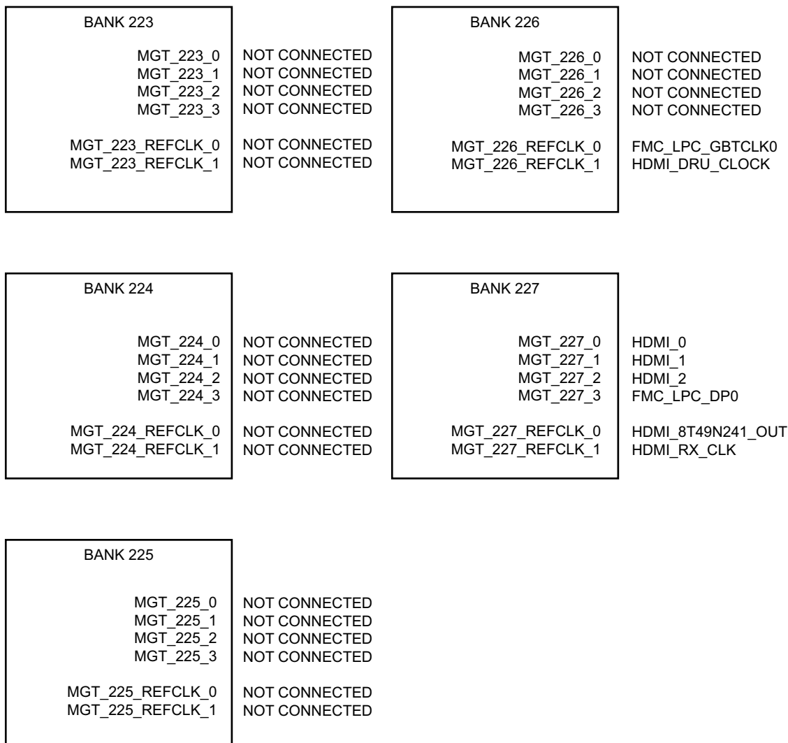
Figure 3-26: GTH Transceiver Bank Assignments
