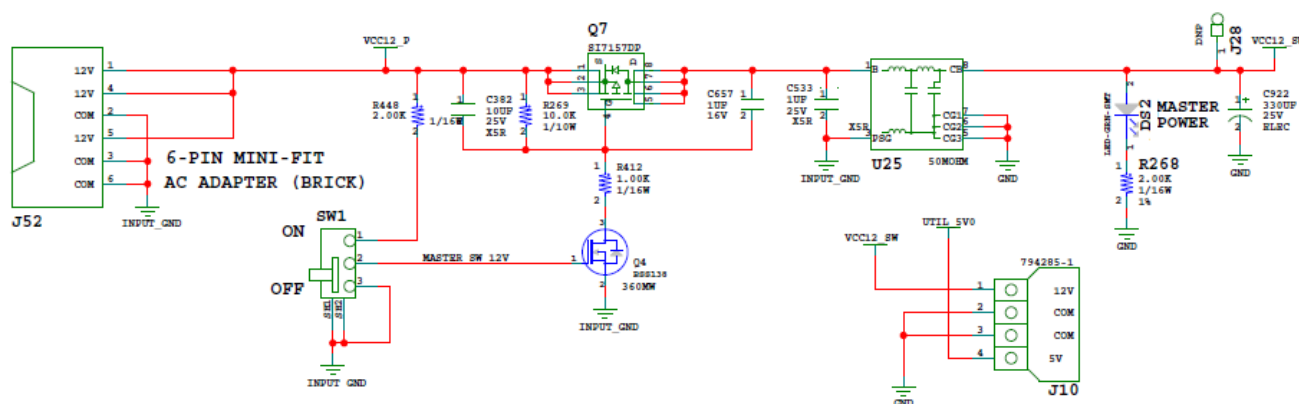
Figure 3-29: Power Input
