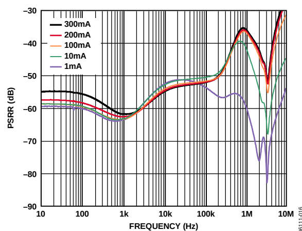
Figure 14. Power Supply Rejection Ratio vs. Frequency, V_{OUT} = 1.8 V
