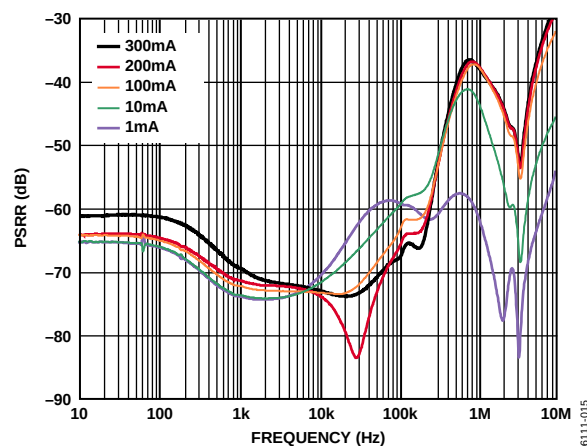
Figure 13. Power Supply Rejection Ratio vs. Frequency, V_{OUT} = 0.8 V
