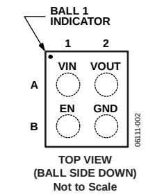
Figure 2. Pin Configuration
