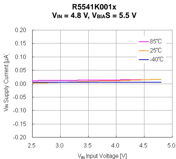
V_{IN} Supply Current vs. V_{IN} Input Voltage
