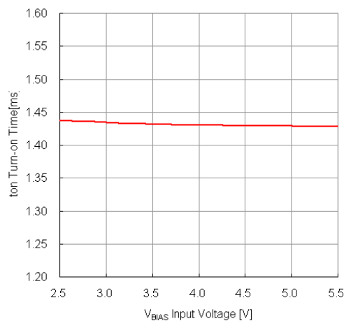
t_{on} Turn-on Time vs. V_{BIAS} Input Voltage
