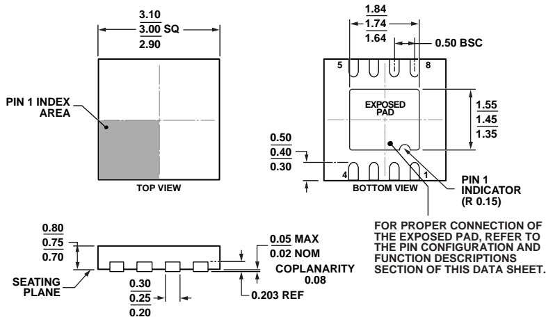
COMPLIANT TO JEDEC STANDARDS MO-229-WEED Figure 73. 8-Lead Lead Frame Chip Scale Package [LFCSF_WD] 3 mm x 3 mm Body, Very Very Thin, Dual Lead (CP-8-13)
