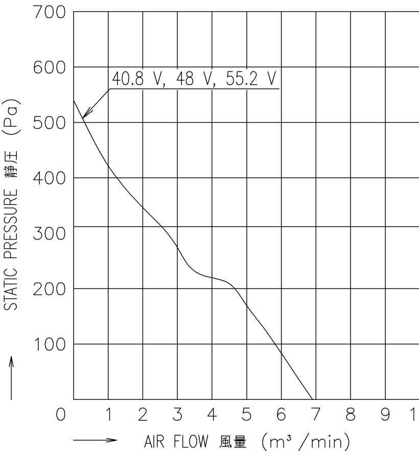
PERFORMANCE CURVES 風量－静圧特性例
