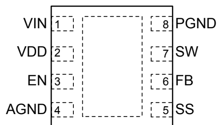
8-Pin 2mm x 2mm MLF ® (ML)
