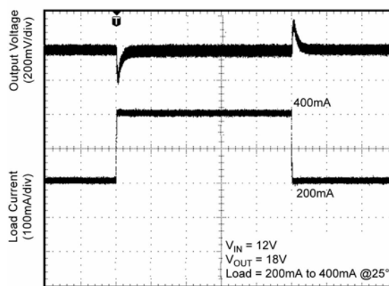
Load Transient
